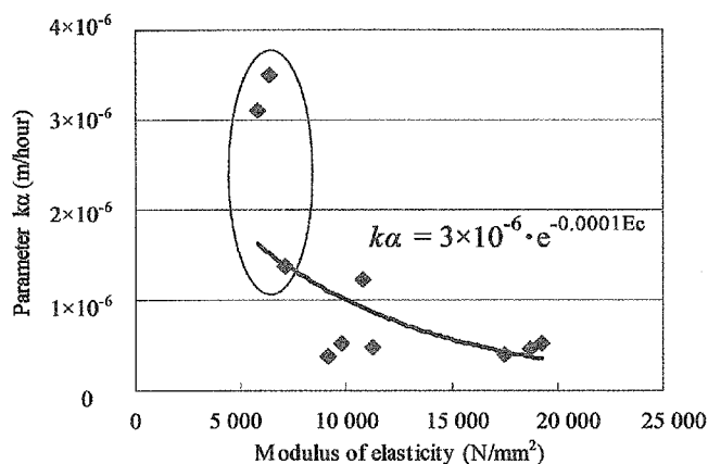
Fig. 5 Relationship between parameter k_{\alpha} and modulus of elasticity.
