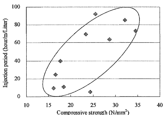
Fig. 1 Relation between compressive strength and injection period.
