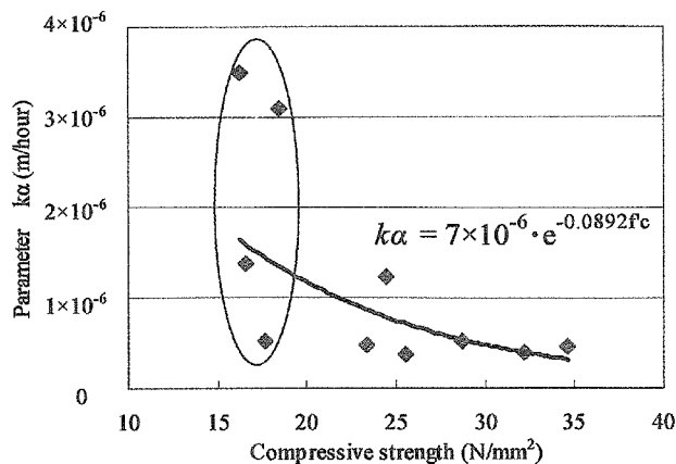
Fig. 4 Relationship between parameter k_{\alpha} and compressive strength.
