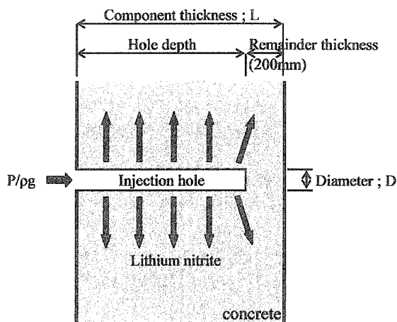
Fig. 3 Pressurized injection outline figure. (Concrete sectional view)
