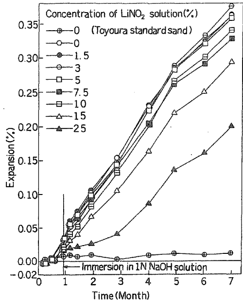
Fig. 10. Expansion of mortars using processed reactive sand particles immersed in 1N NaOH solution at 20°C (B series).
